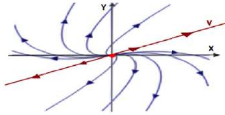
Figura 7.9: Nodo impropio inestable
