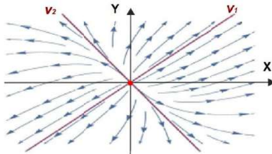
Figura 7.4: Nodo inestable
